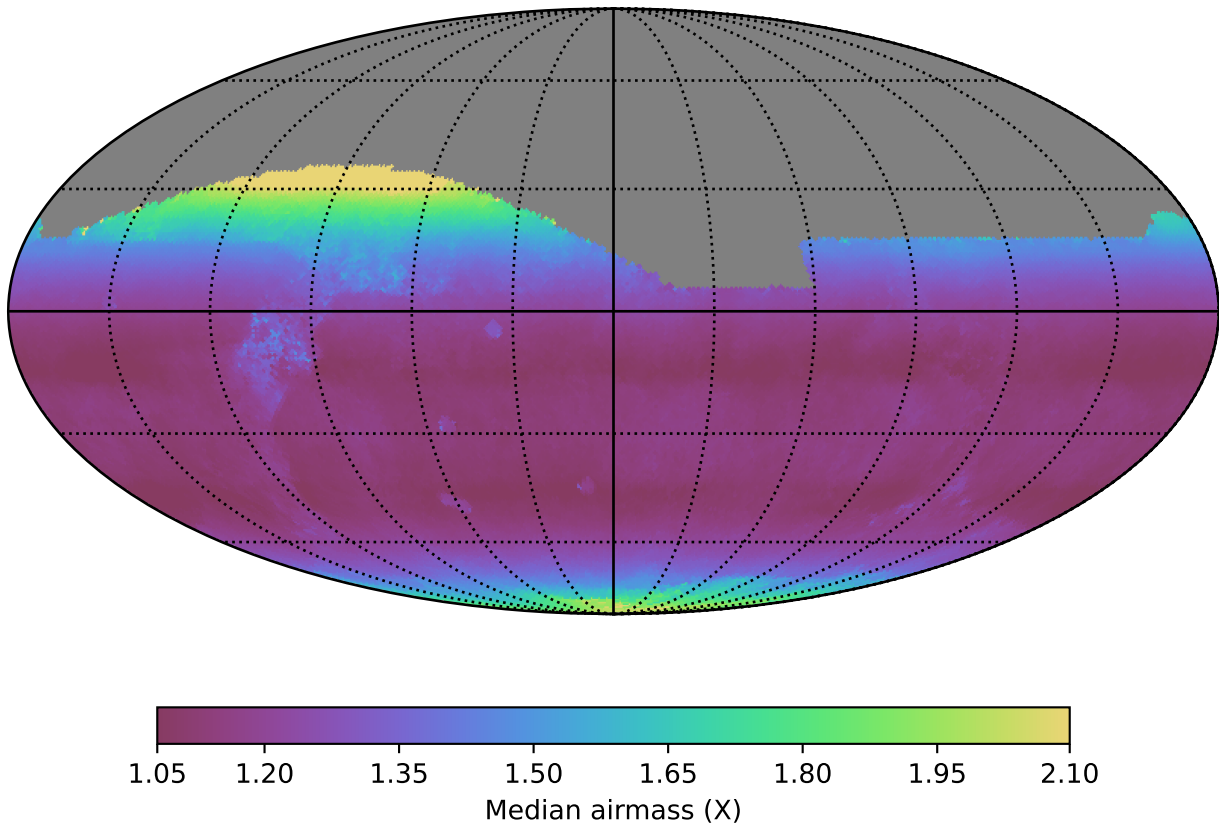
too_10_4v3.4_10yrs All sky i band: Median airmass
