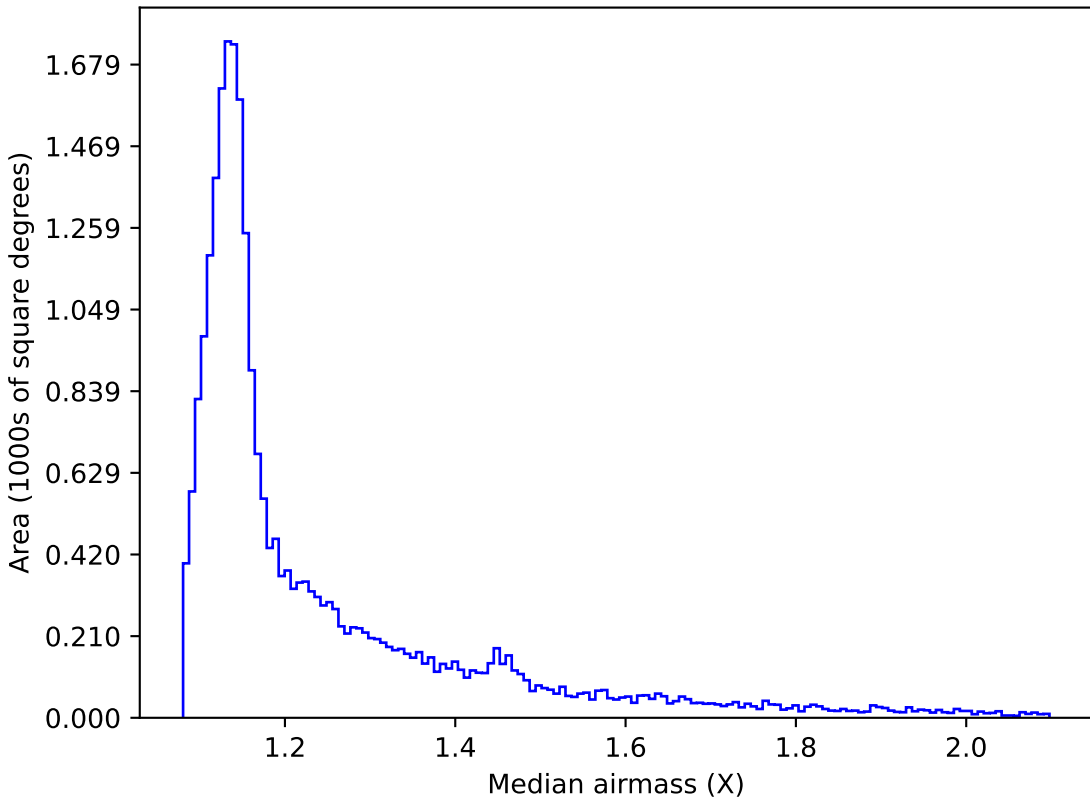
too_10_4v3.4_10yrs All sky i band: Median airmass
