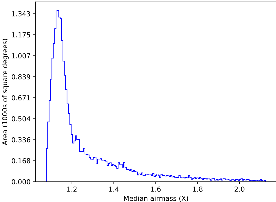
too_10_4v3.4_10yrs All sky g band: Median airmass
