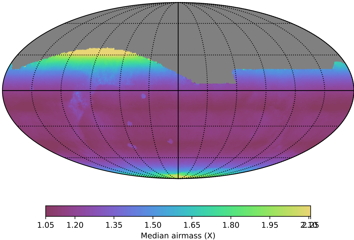
too_10_4v3.4_10yrs All sky all bands: Median airmass
