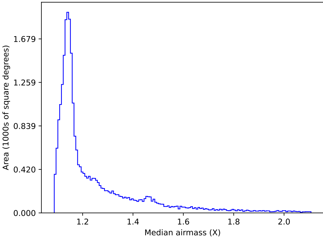
too_10_4v3.4_10yrs All sky all bands: Median airmass
