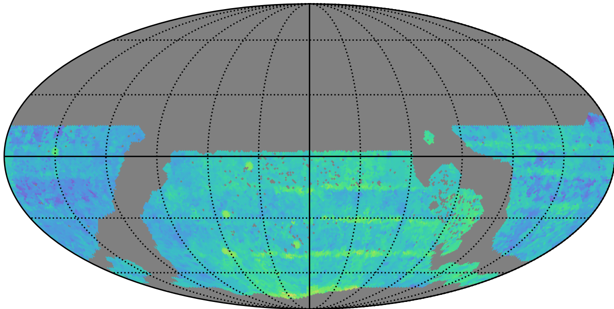
too_10_4v3.4_10yrs WFD z band: Median Season Length
