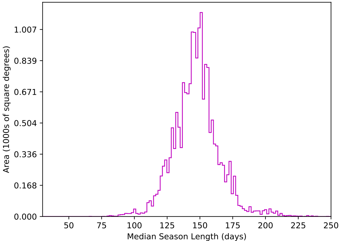
too_10_4v3.4_10yrs WFD z band: Median Season Length
