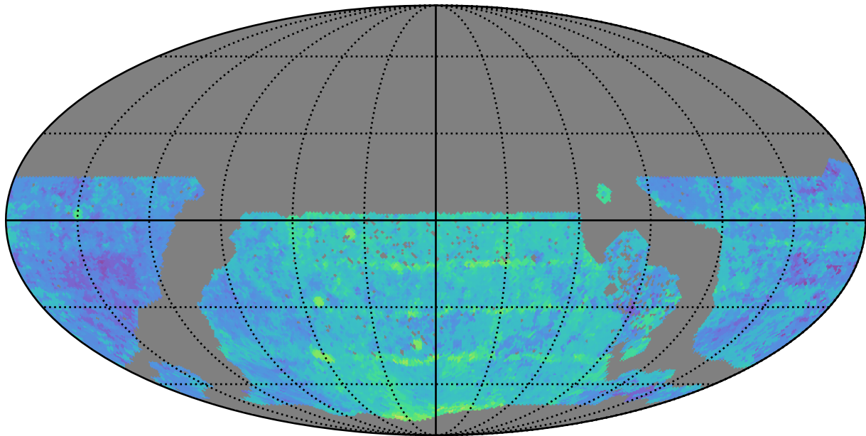
too_10_4v3.4_10yrs WFD y band: Median Season Length
