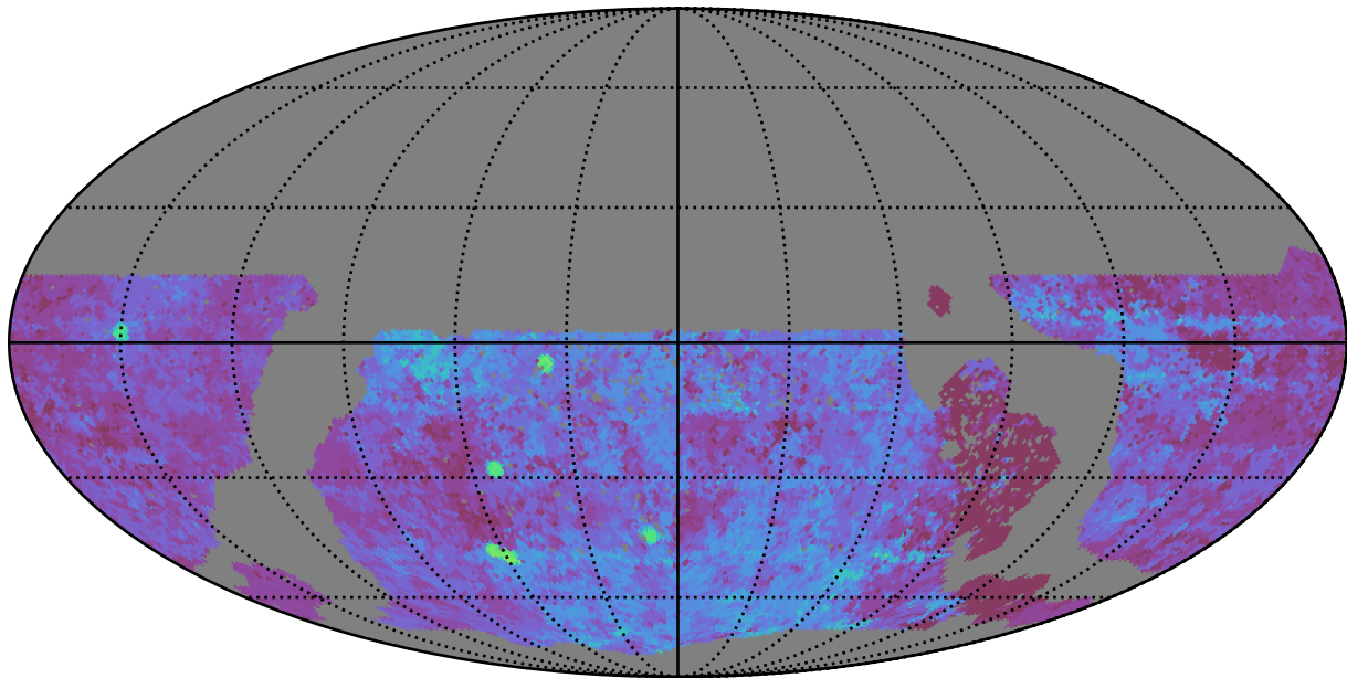
too_10_4v3.4_10yrs WFD u band: Median Season Length
