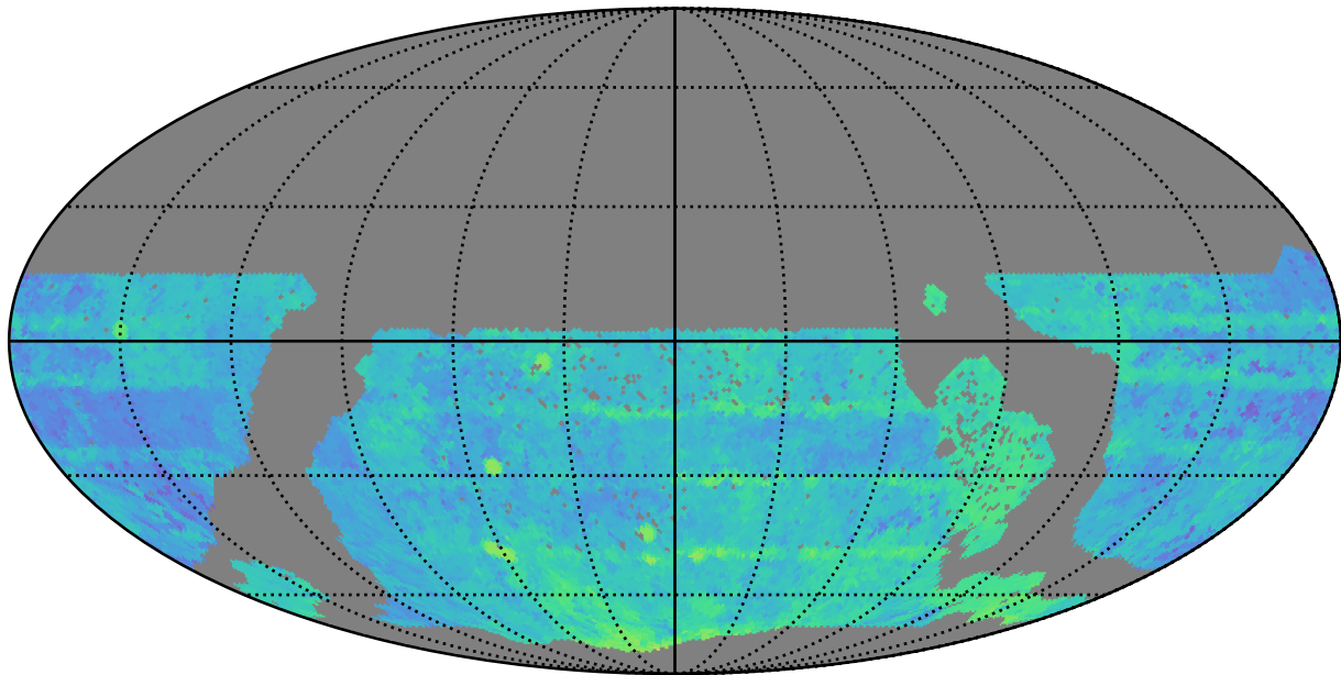
too_10_4v3.4_10yrs WFD r band: Median Season Length
