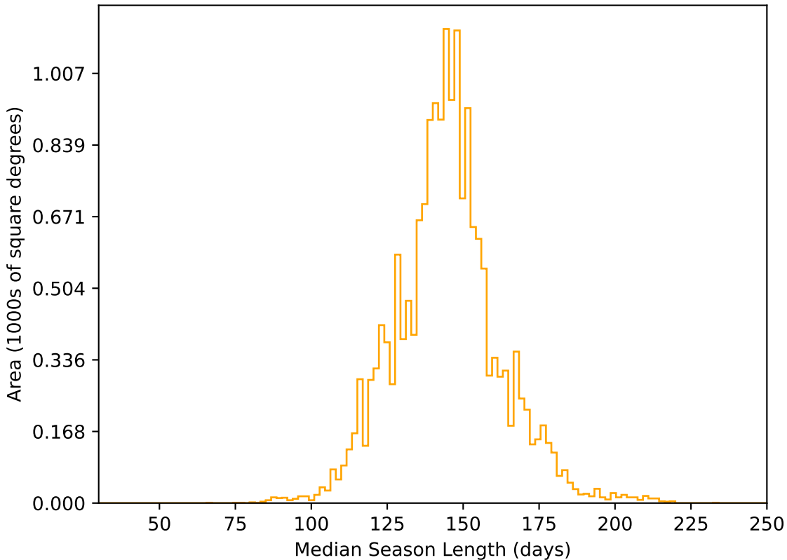
too_10_4v3.4_10yrs WFD r band: Median Season Length
