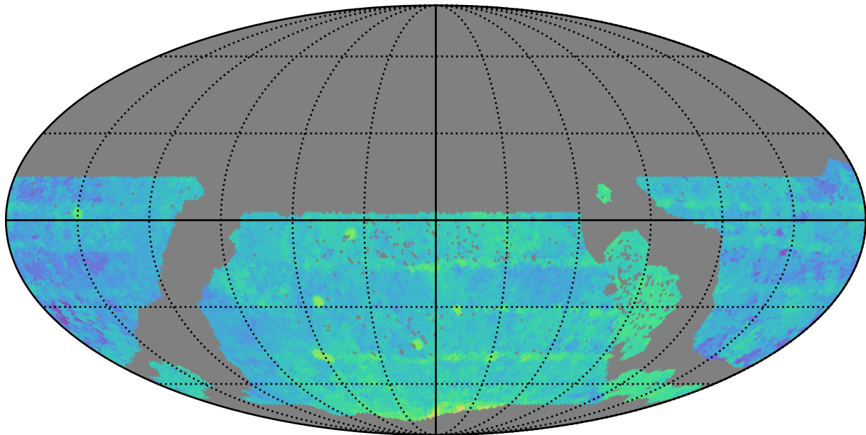
too_10_4v3.4_10yrs WFD i band: Median Season Length
