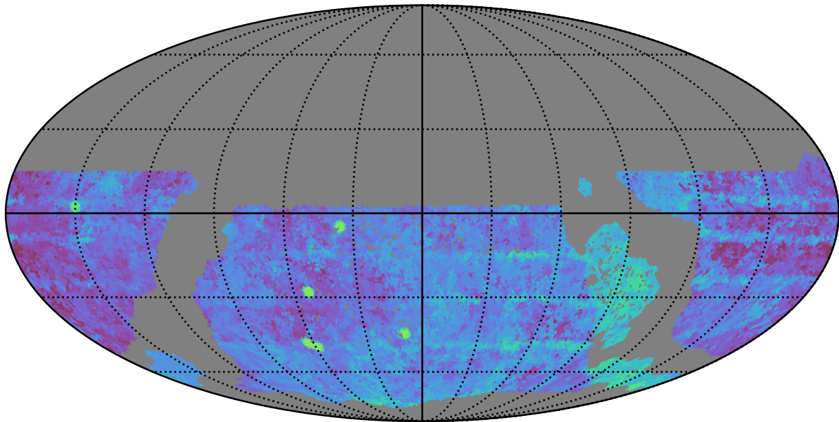
too_10_4v3.4_10yrs WFD g band: Median Season Length
