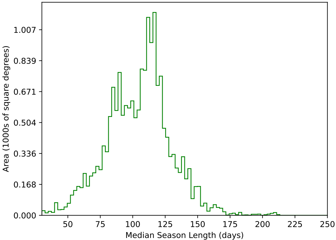
too_10_4v3.4_10yrs WFD g band: Median Season Length
