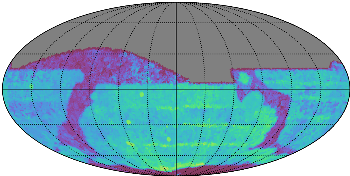
too_10_4v3.4_10yrs All sky z band: Median Season Length
