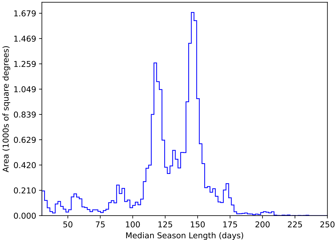
too_10_4v3.4_10yrs All sky y band: Median Season Length
