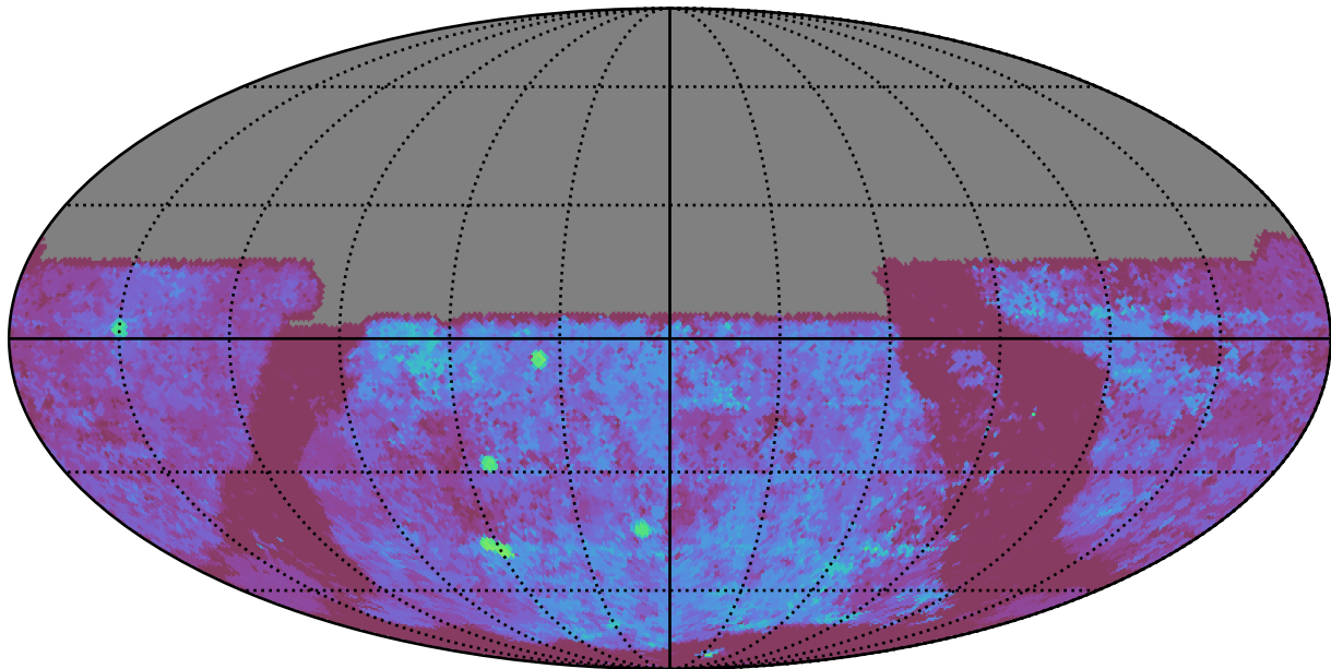
too_10_4v3.4_10yrs All sky u band: Median Season Length
