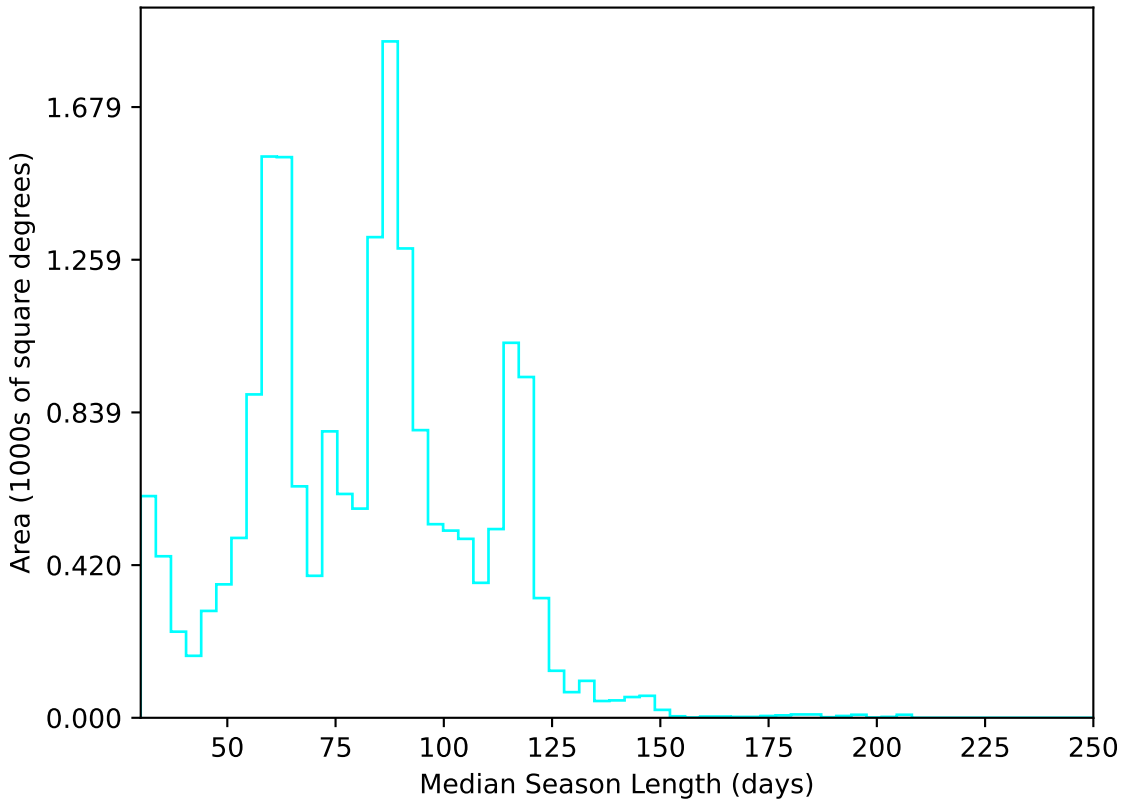
too_10_4v3.4_10yrs All sky u band: Median Season Length
