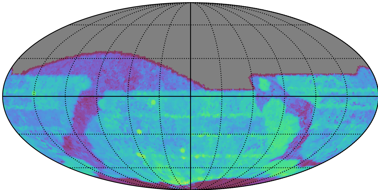
too_10_4v3.4_10yrs All sky r band: Median Season Length
