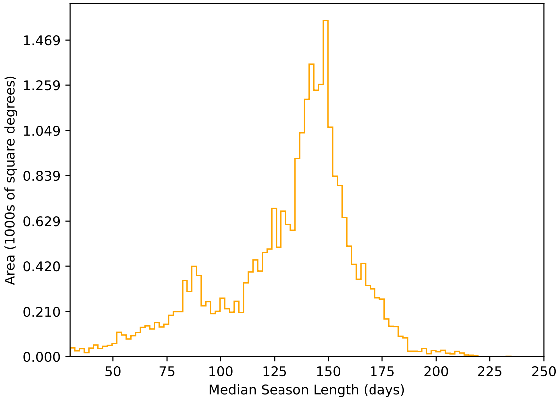
too_10_4v3.4_10yrs All sky r band: Median Season Length
