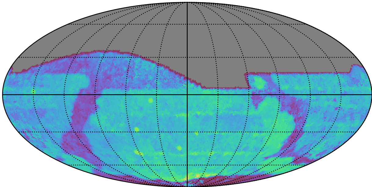
too_10_4v3.4_10yrs All sky i band: Median Season Length
