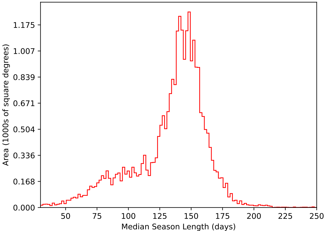
too_10_4v3.4_10yrs All sky i band: Median Season Length
