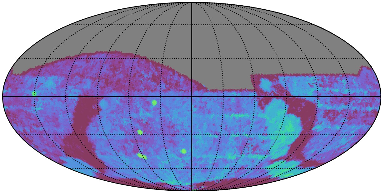
too_10_4v3.4_10yrs All sky g band: Median Season Length
