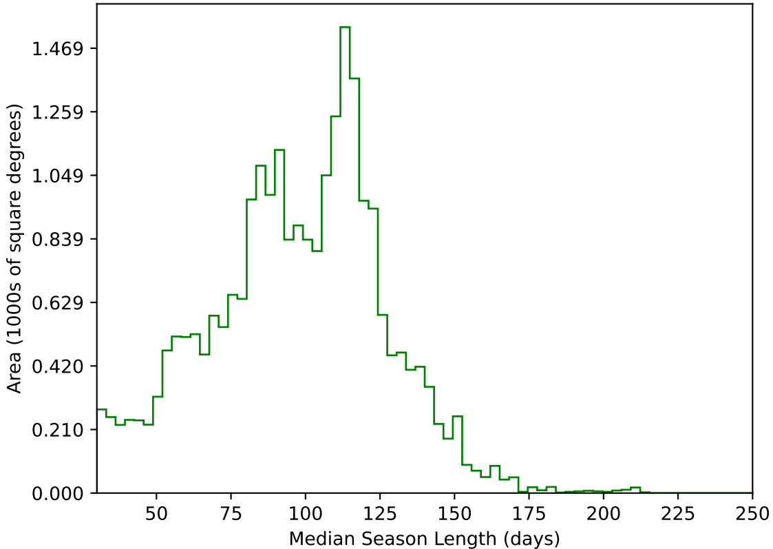
too_10_4v3.4_10yrs All sky g band: Median Season Length
