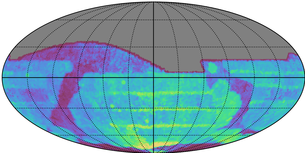
too_10_4v3.4_10yrs All sky all bands: Median Season Length
