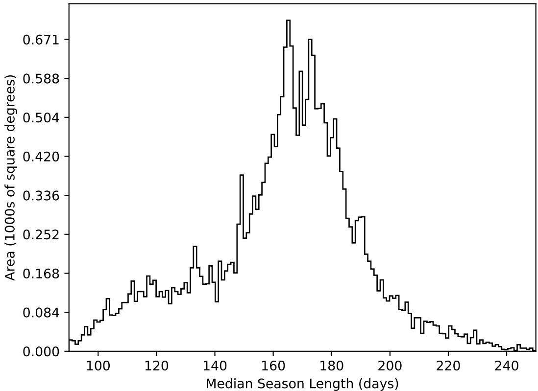
too_10_4v3.4_10yrs All sky all bands: Median Season Length
