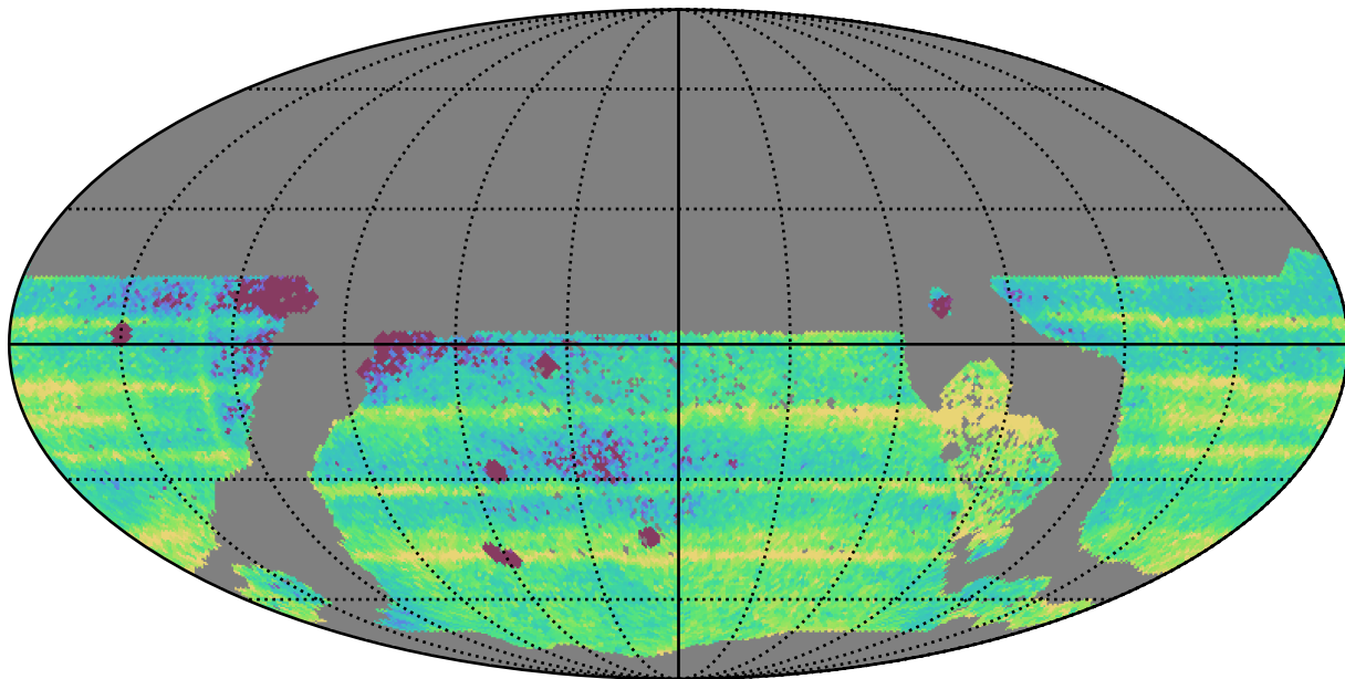
too_10_4v3.4_10yrs WFD: Median Intra-Night Gap
