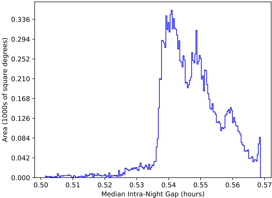
too_10_4v3.4_10yrs WFD: Median Intra-Night Gap
