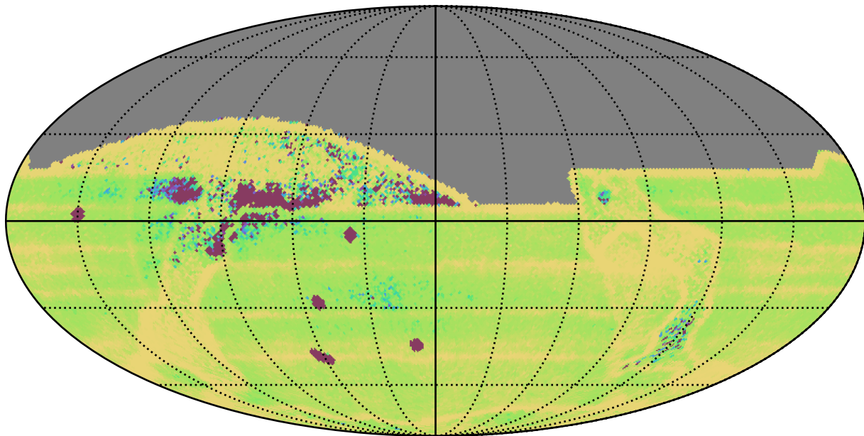
too_10_4v3.4_10yrs All sky: Median Intra-Night Gap
