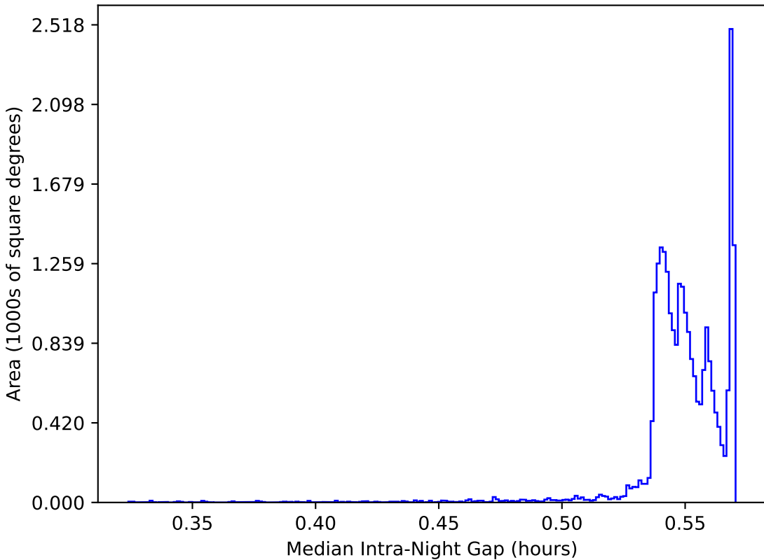
too_10_4v3.4_10yrs All sky: Median Intra-Night Gap
