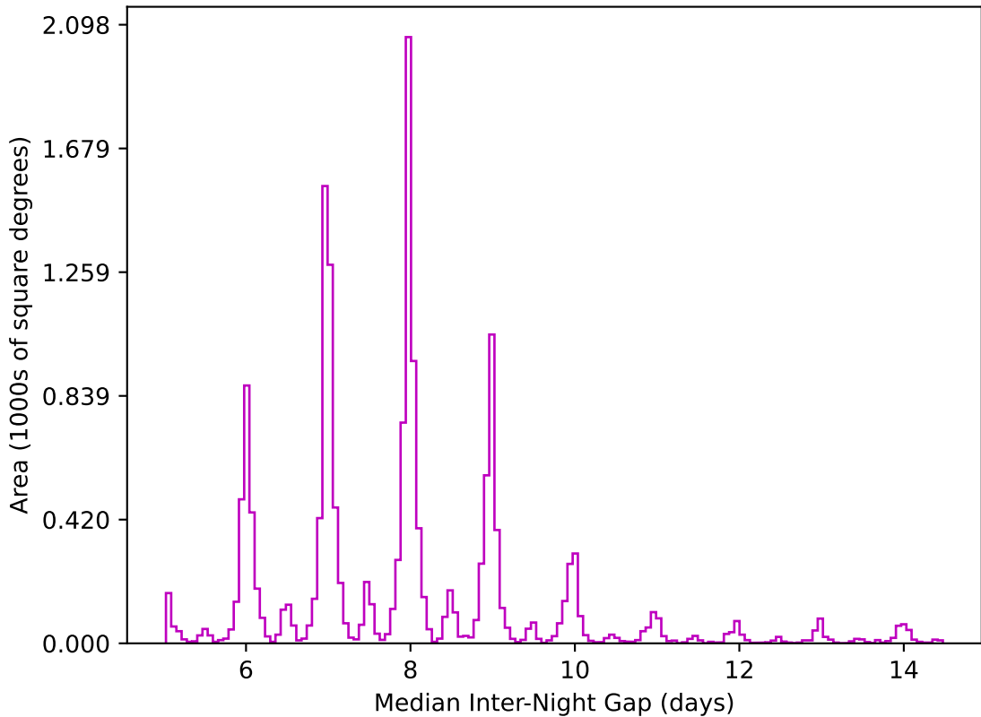
too_10_4v3.4_10yrs WFD z band: Median Inter-Night Gap
