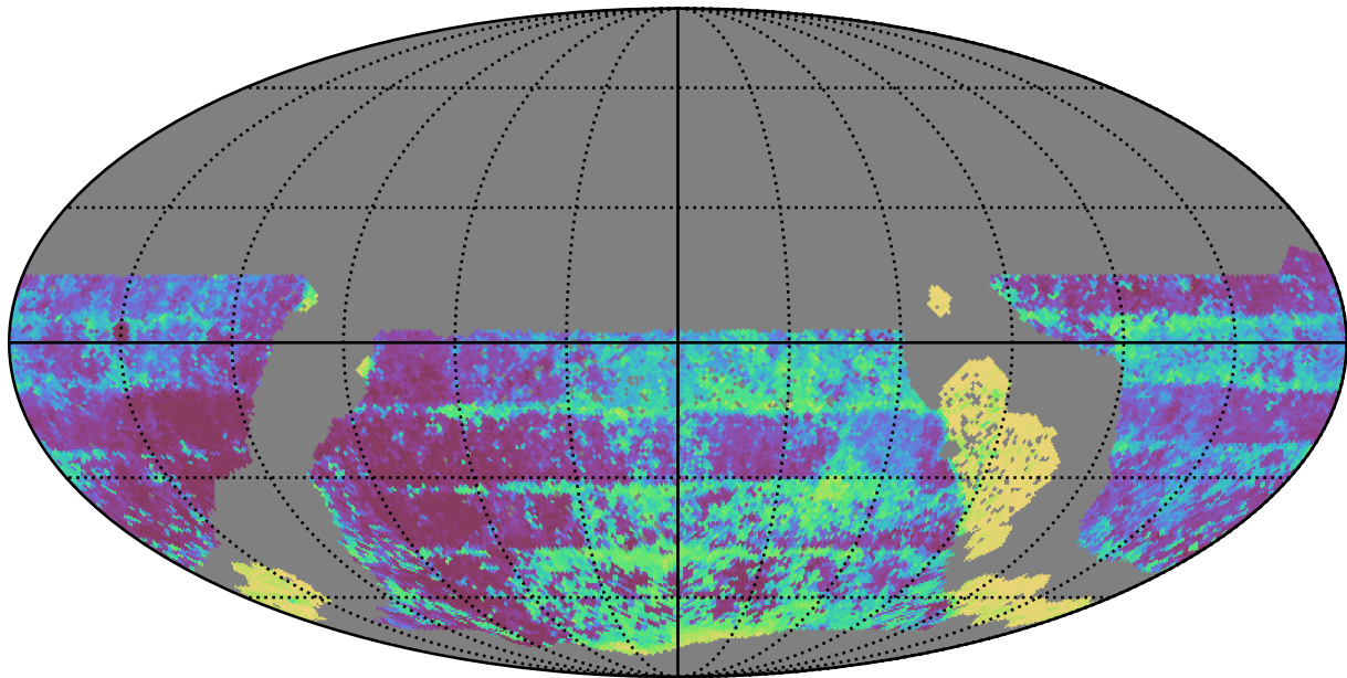
too_10_4v3.4_10yrs WFD y band: Median Inter-Night Gap
