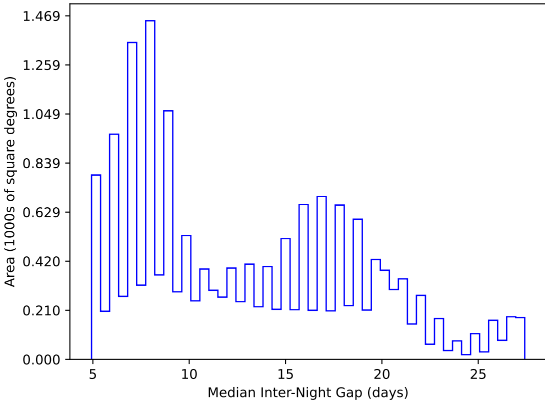
too_10_4v3.4_10yrs WFD y band: Median Inter-Night Gap
