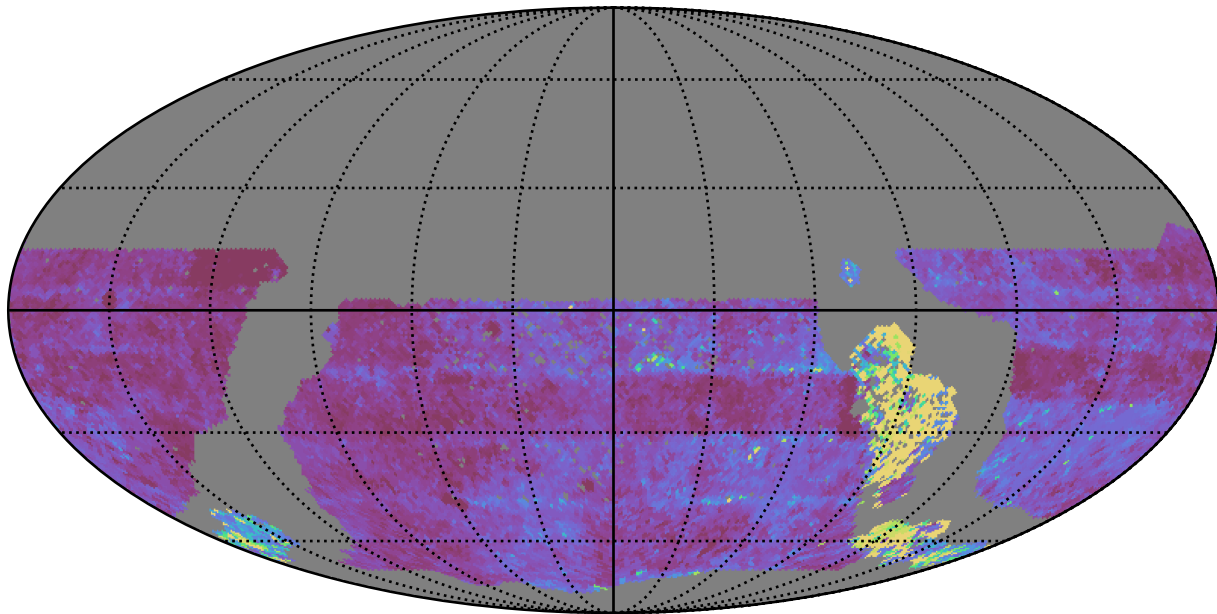
too_10_4v3.4_10yrs WFD u band: Median Inter-Night Gap
