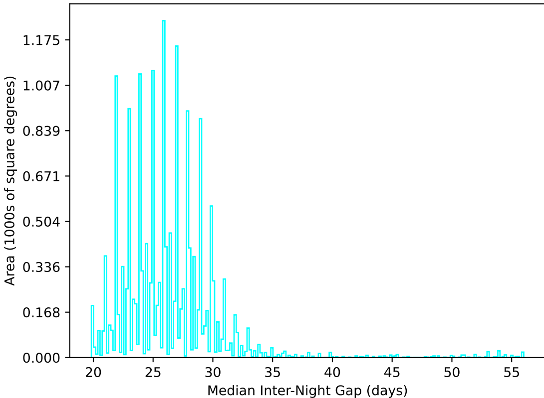
too_10_4v3.4_10yrs WFD u band: Median Inter-Night Gap
