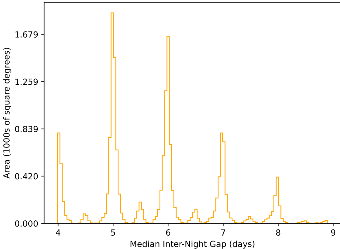
too_10_4v3.4_10yrs WFD r band: Median Inter-Night Gap
