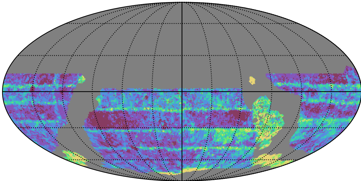
too_10_4v3.4_10yrs WFD i band: Median Inter-Night Gap
