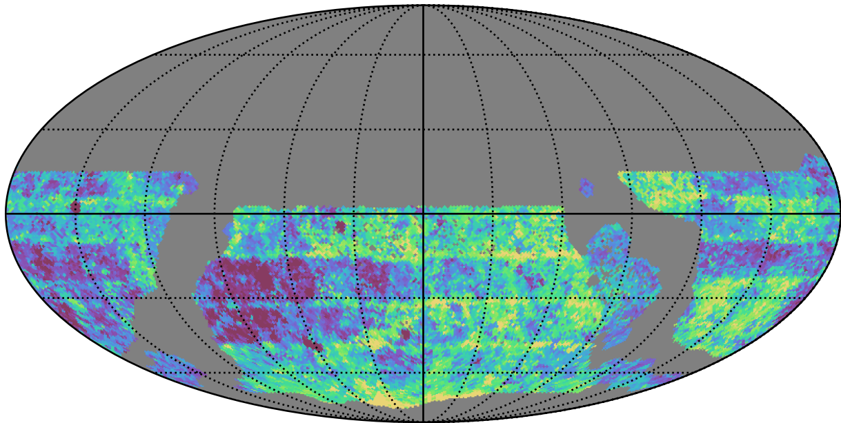
too_10_4v3.4_10yrs WFD g band: Median Inter-Night Gap
