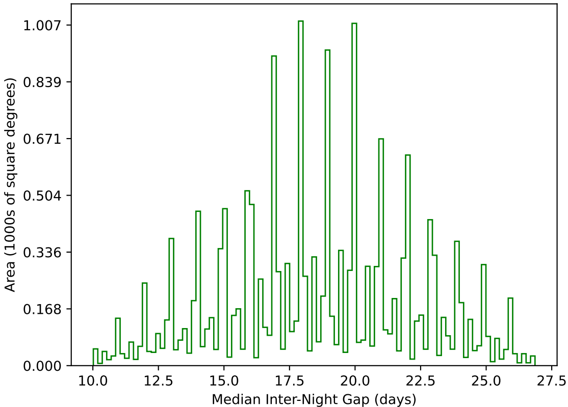
too_10_4v3.4_10yrs WFD g band: Median Inter-Night Gap
