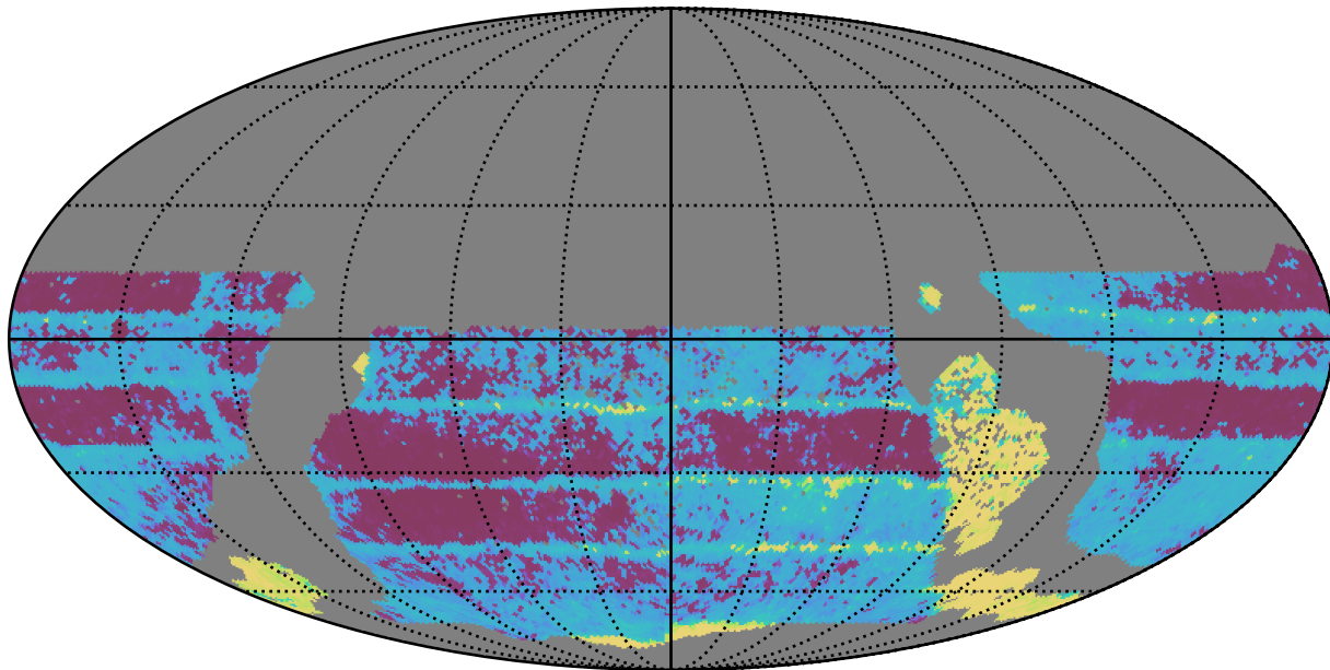
too_10_4v3.4_10yrs WFD all bands: Median Inter-Night Gap
