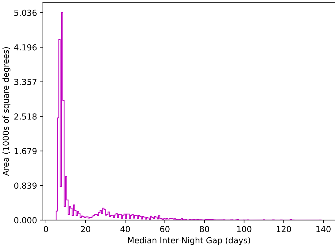
too_10_4v3.4_10yrs All sky z band: Median Inter-Night Gap
