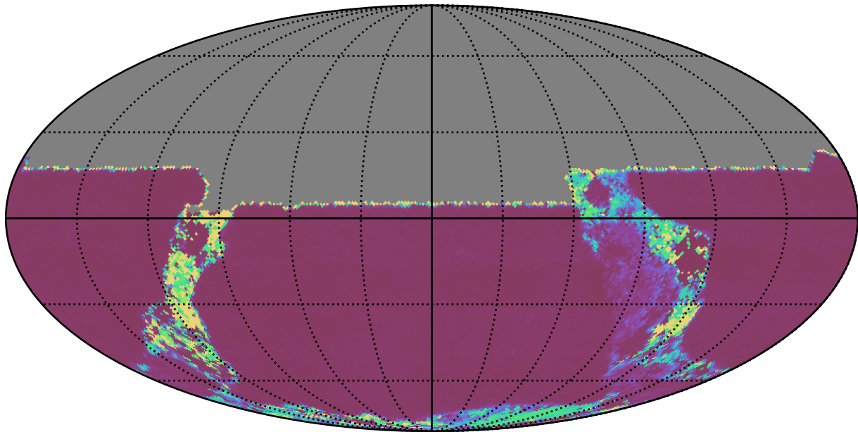
too_10_4v3.4_10yrs All sky u band: Median Inter-Night Gap
