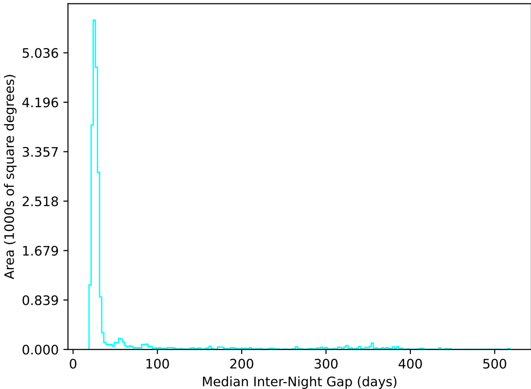
too_10_4v3.4_10yrs All sky u band: Median Inter-Night Gap
