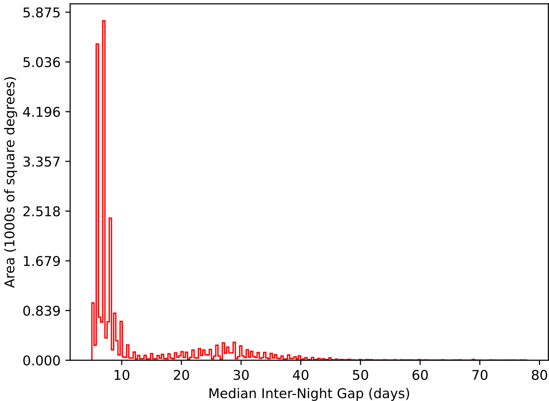
too_10_4v3.4_10yrs All sky i band: Median Inter-Night Gap
