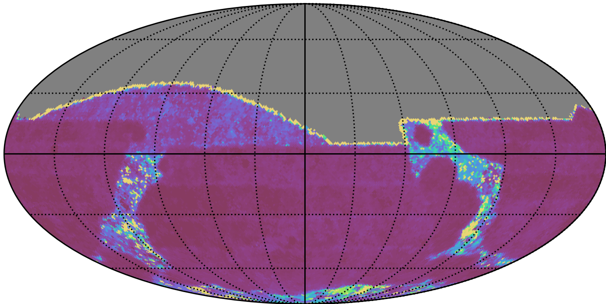
too_10_4v3.4_10yrs All sky g band: Median Inter-Night Gap
