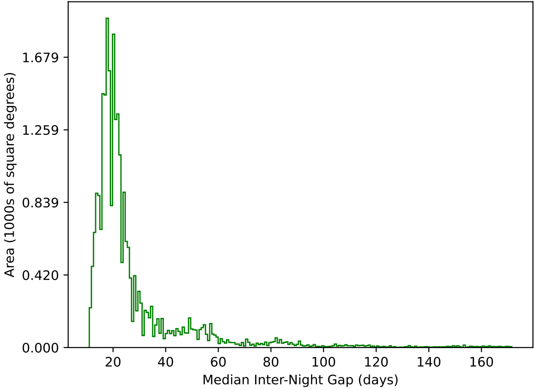
too_10_4v3.4_10yrs All sky g band: Median Inter-Night Gap
