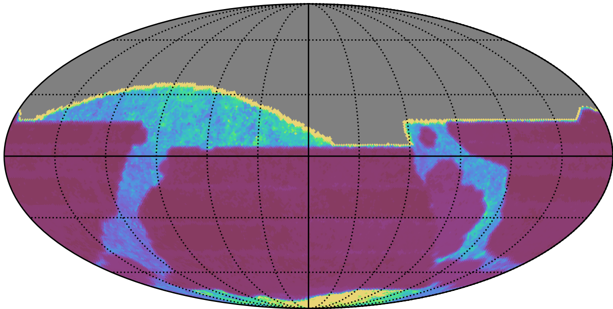
too_10_4v3.4_10yrs All sky all bands: Median Inter-Night Gap
