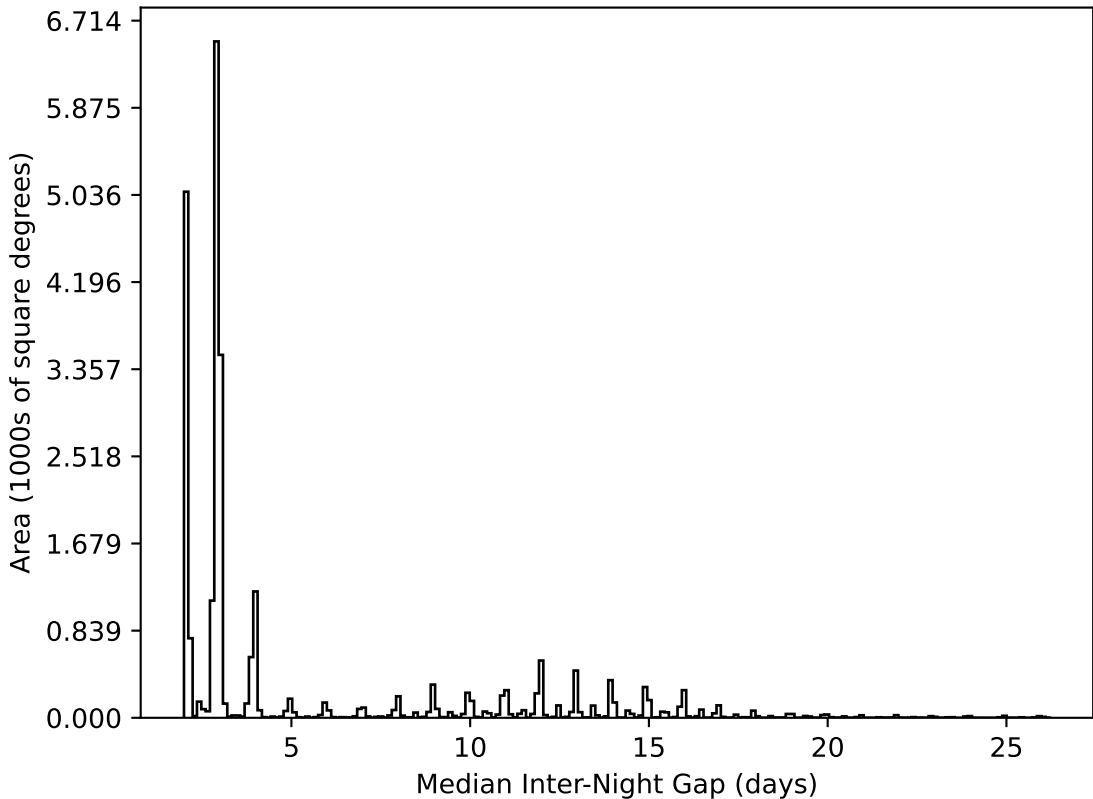
too_10_4v3.4_10yrs All sky all bands: Median Inter-Night Gap
