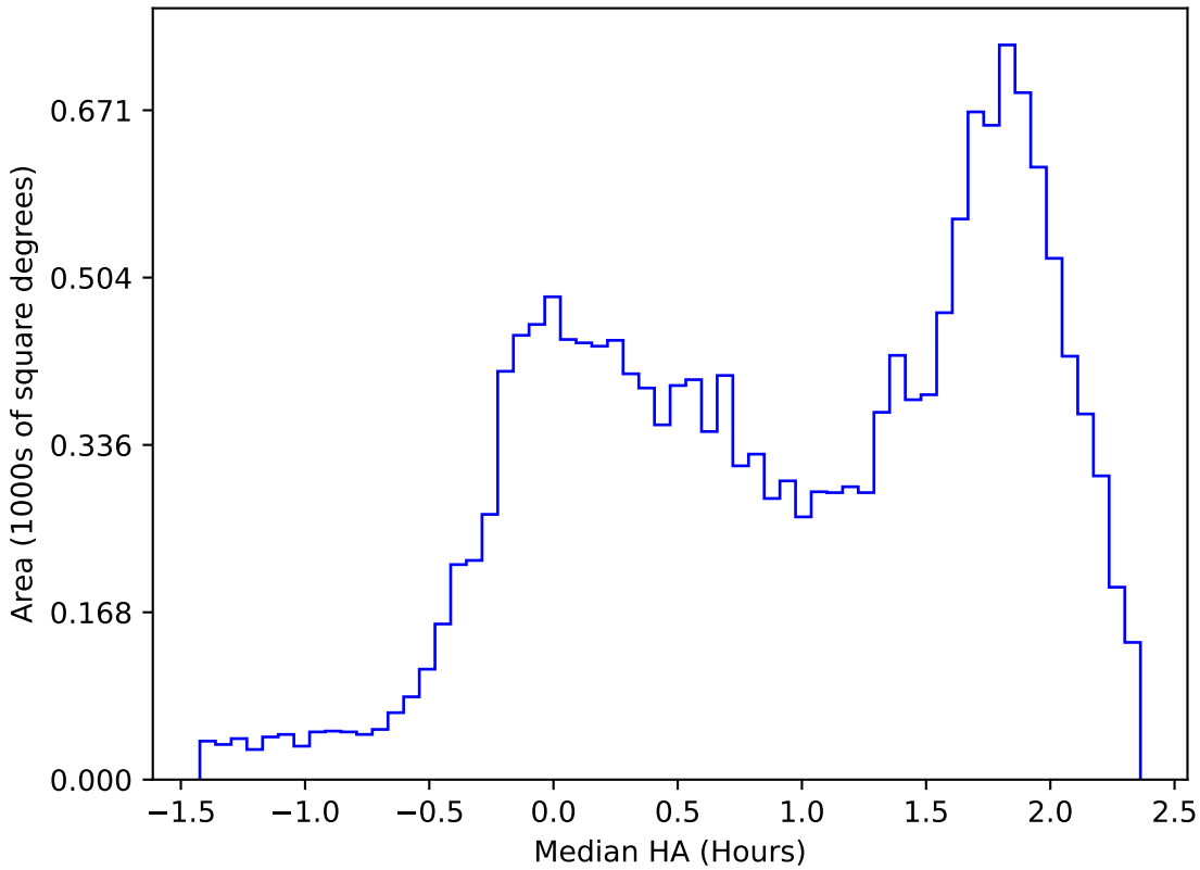
too_10_4v3.4_10yrs WFD u band: Median HA
