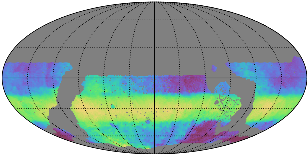
too_10_4v3.4_10yrs WFD r band: Median HA
